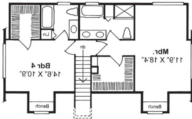
Plan Number 34077 | Order Code: GOEXP | Second Floor Plan
